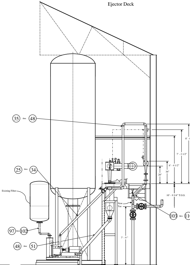
Elevation View B-B Evaporator Mezzanine (Looking North)
