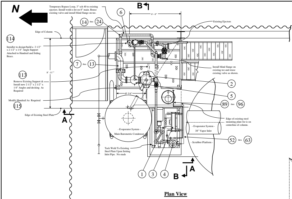
Plan View Evaporator Mezzanine
