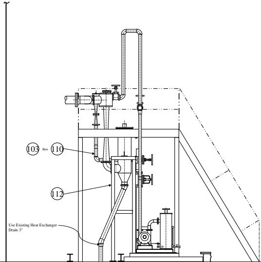
Elevation View A-A Evaporator Mezzanine (Looking East)
