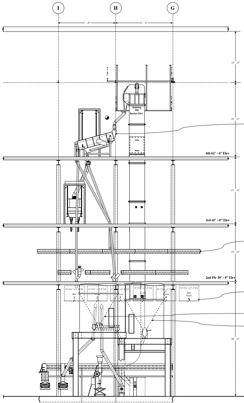
ELEVATION VIEW Looking South
