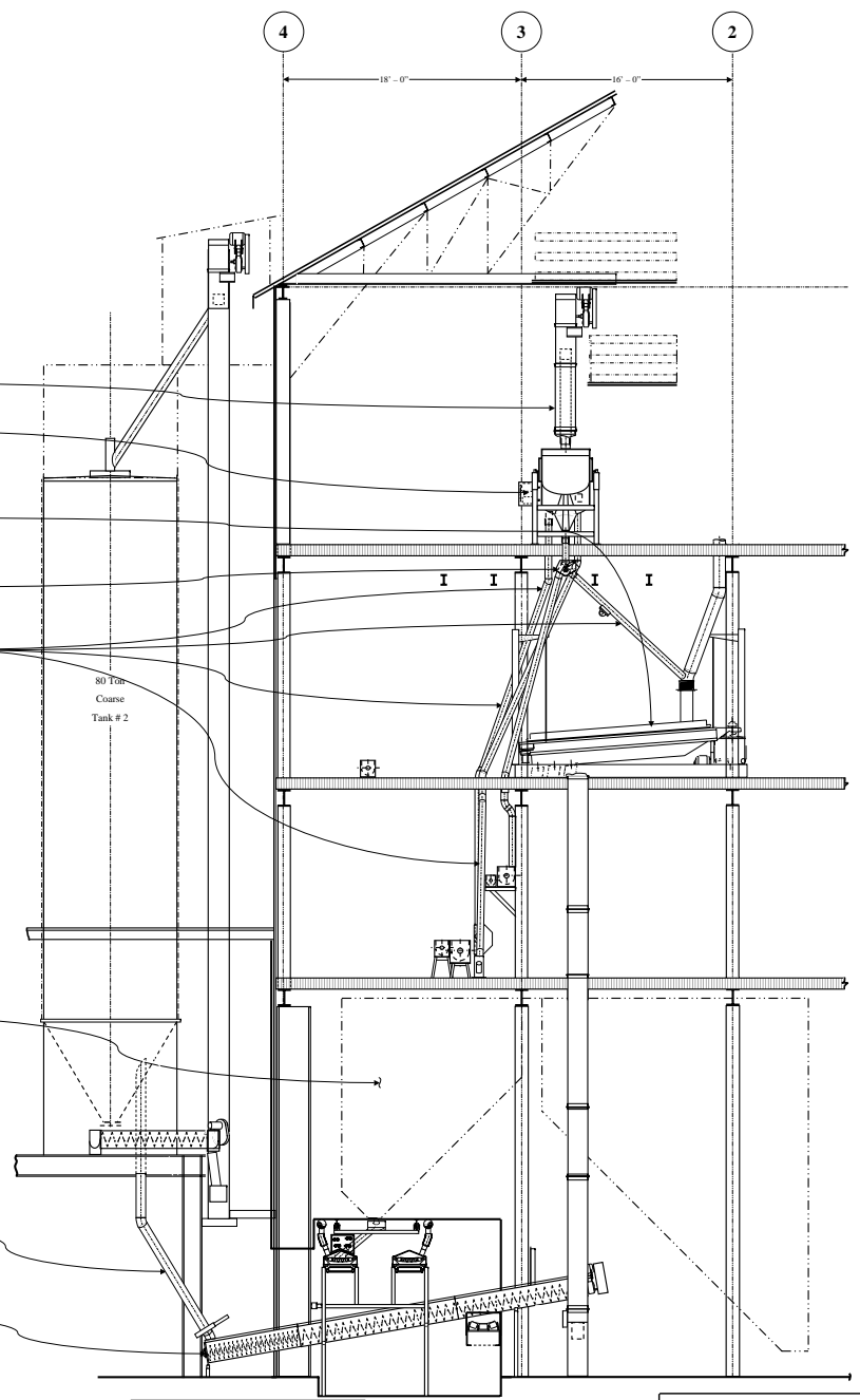
ELEVATION VIEW Looking East
